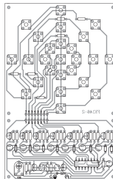
Figure 2. Circuit Assembling
