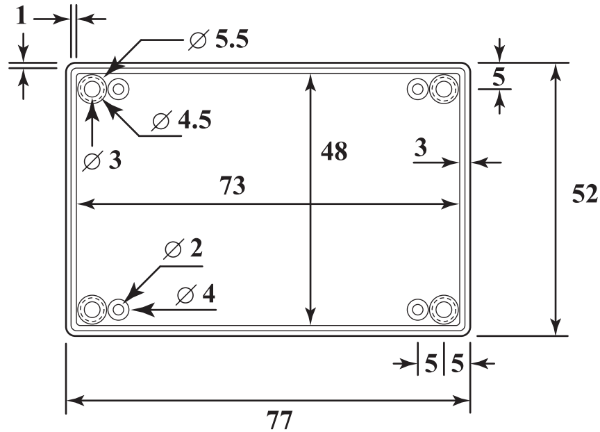
Bottom View
